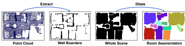
Fig. 15: Visualization of room segmentation process.
